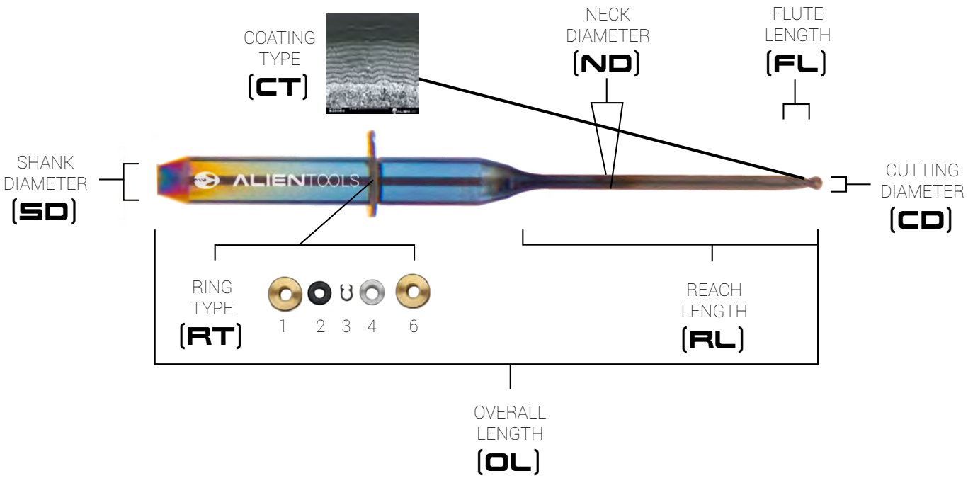
BALL-NOSE TOOL, FLAT COAT™ REAL DIAMOND COATING, FOR MILLING ZIRCONIA (SIZES IN MM, PRICES EXCLUDING VAT)
