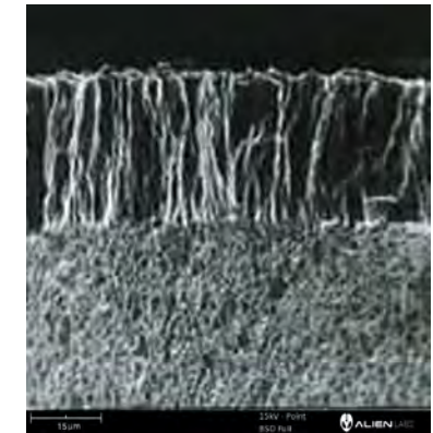
Side View of Regular Coating
